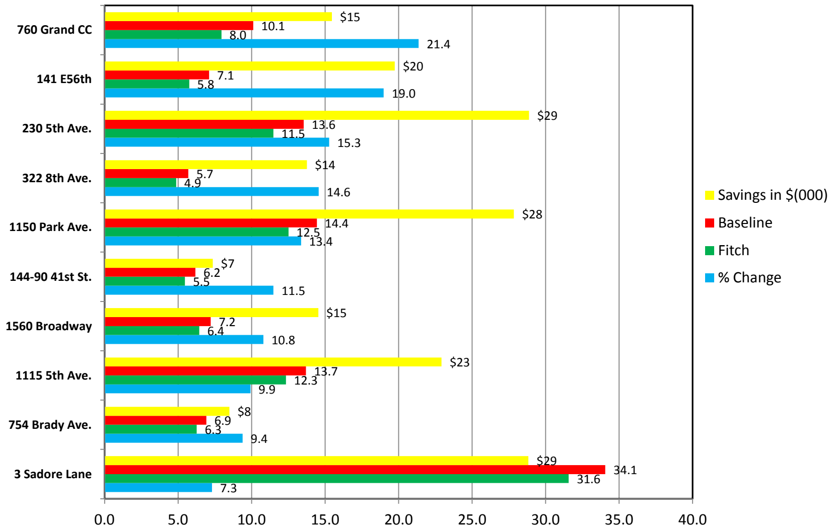
Gallon per degree day fuel oil comparison with Fitch Fuel Catalyst Estimated Annual Fuel Savings in Thousands of Dollars
